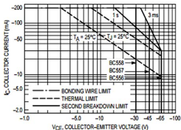
Fig 14: Active Region — Safe Operating Area
