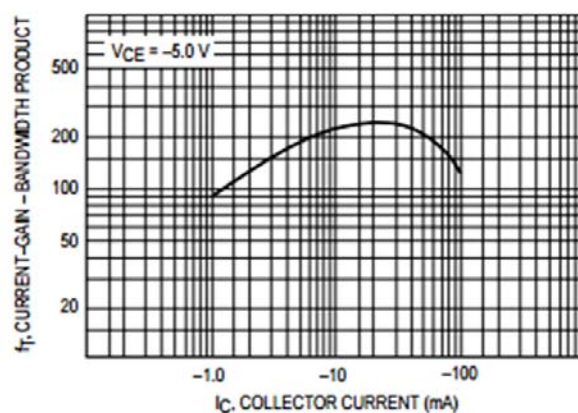
Fig 12: Current-Gain – Bandwidth Product
