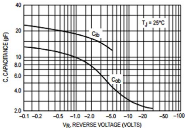
Fig 9: Capacitance
