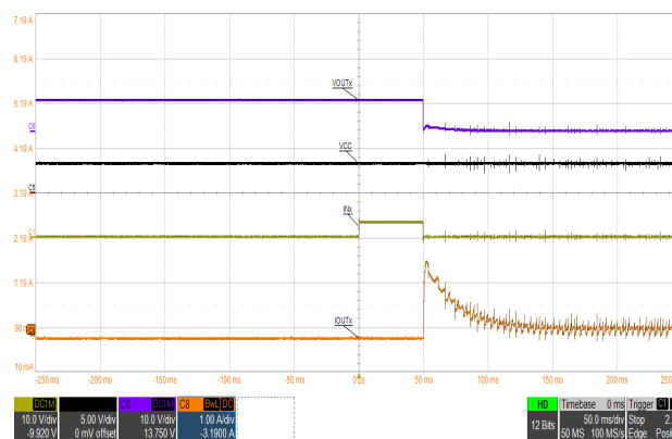
A. Channel 1 = IN1, IN2 (paralleled) Channel 5 = V_{CC} Channel 6 = V_{OUT} (OUT1/2 paralleled) Channel 8 = Motor Current
